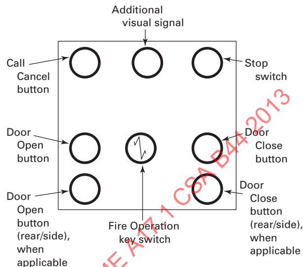
Fig. 2.27.3.3.7 Panel Layout
