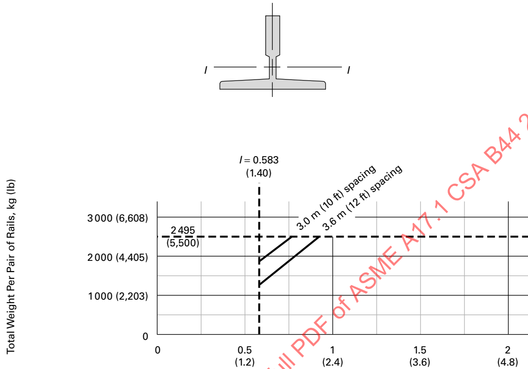
Fig. 2.23.4.1-2 Minimum Moment of Inertia About x-x Axis for a Single Guide Rail With Its Reinforcement
