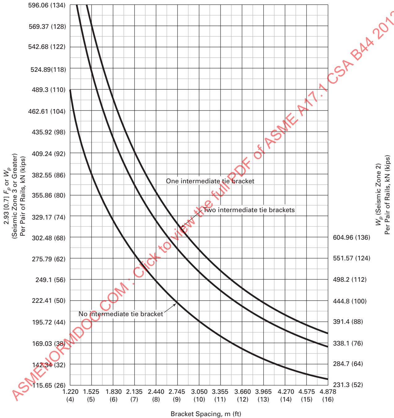
Fig. 8.4.8.2-7 44.5 kg/m (30 lb/ft) Guide-Rail Bracket Spacing
