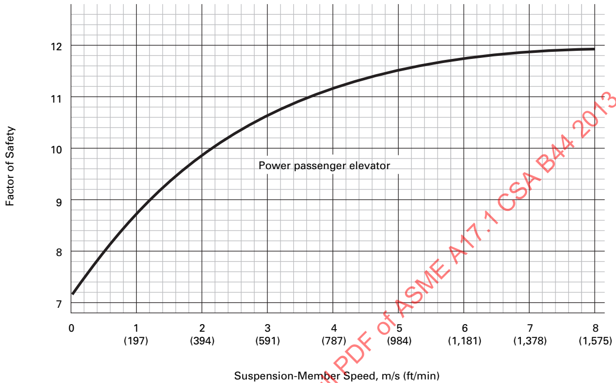
Fig. 8.2.7 Minimum Factors of Safety of Suspension Members of Power Passenger and Freight Elevators
