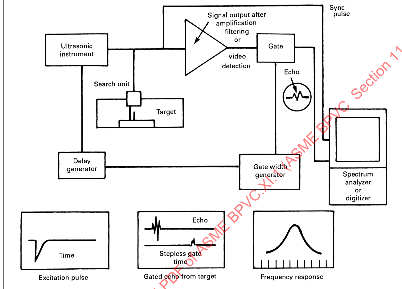
Figure VIII-S1-1A System Configuration
