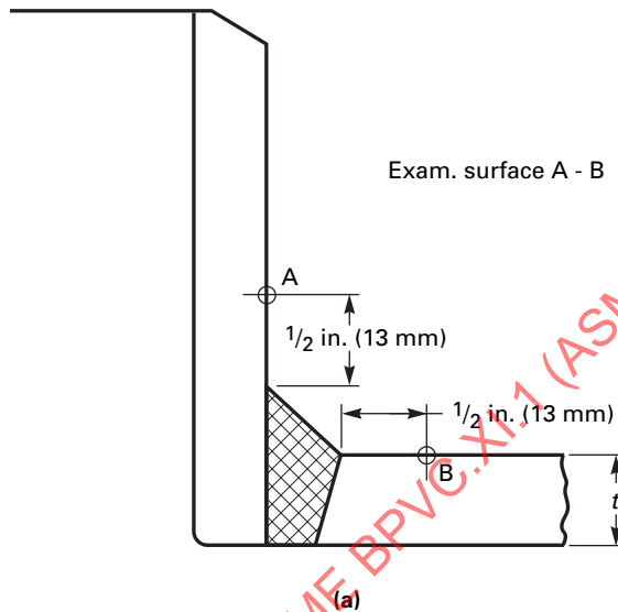
Figure IWC-2500-3 Nozzle-to-Vessel Welds
