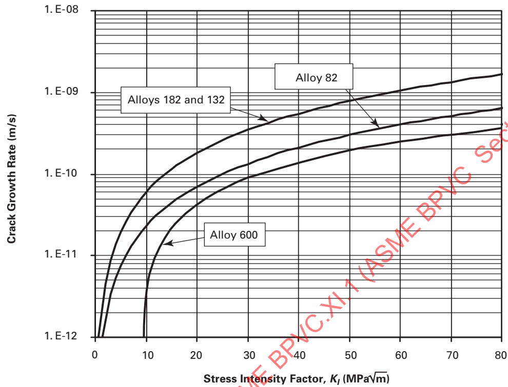
Figure C-8510-1M SCC Curves for Alloy 600, 82, 182, and 132 in PWR Environment at 325°C
