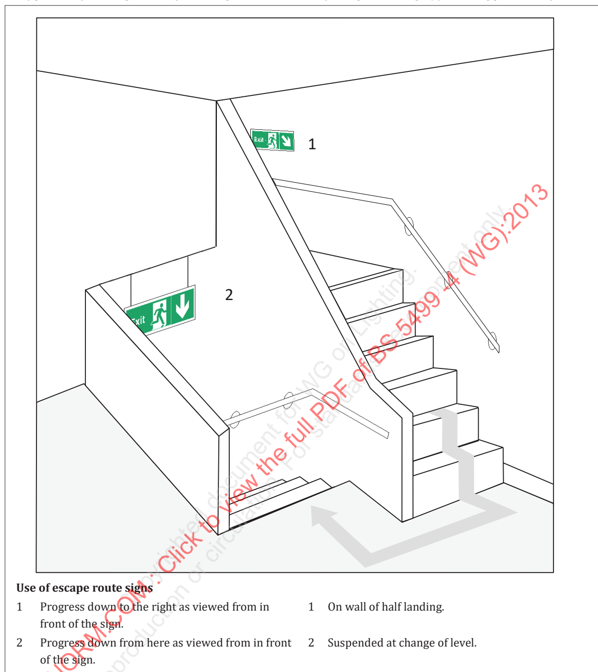
Figure A.3 — Typical half landing stairway showing the correct use of escape route sign(s) with supplementary text
