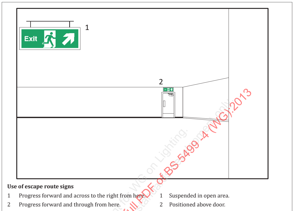
Figure A.17 — Typical large open plan area showing the correct use of escape route sign(s) and supplementary text
