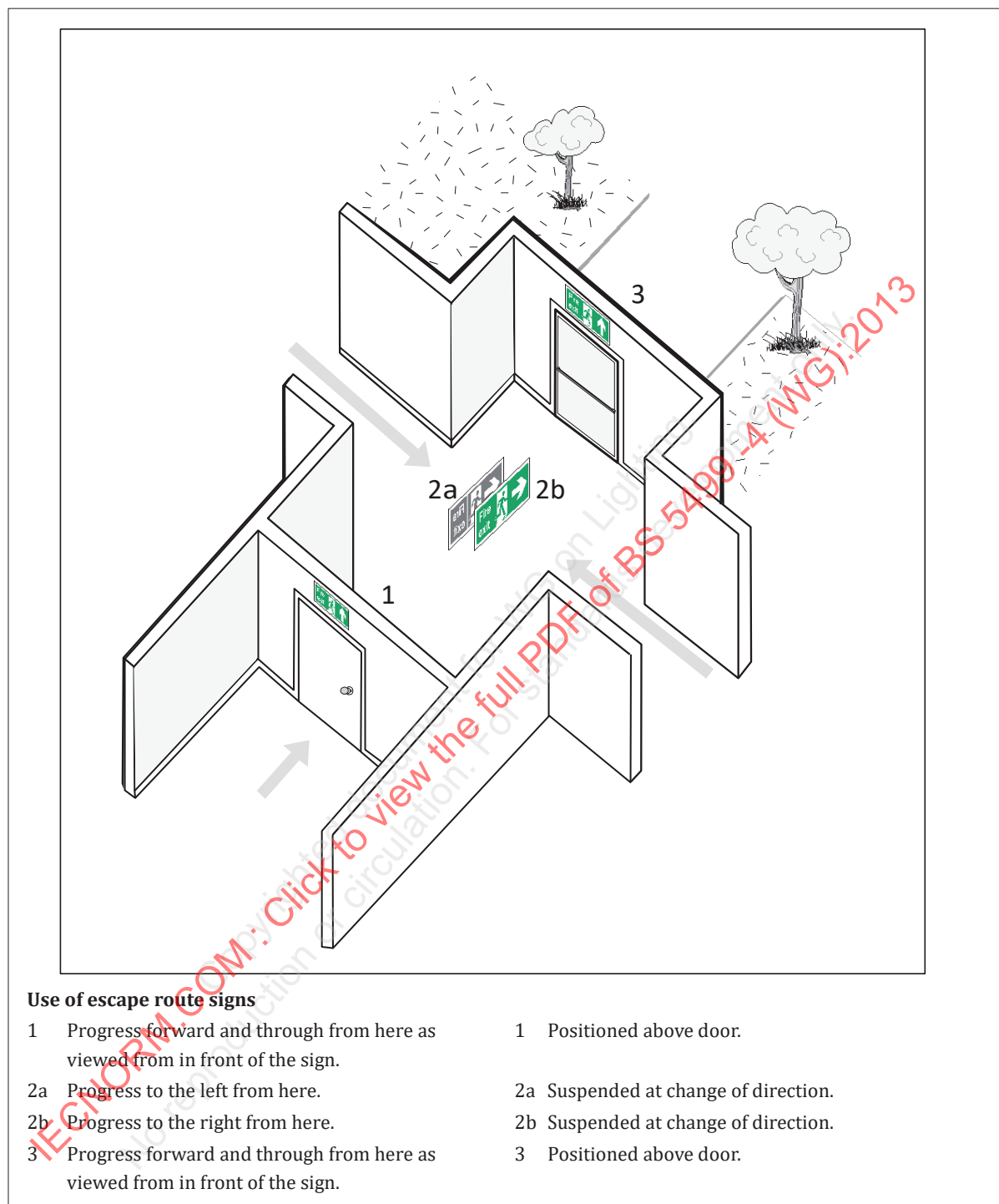
Figure A.5 — Typical cross junction/corridor(s) to final fire exit showing the correct use of escape route sign(s) with supplementary text
