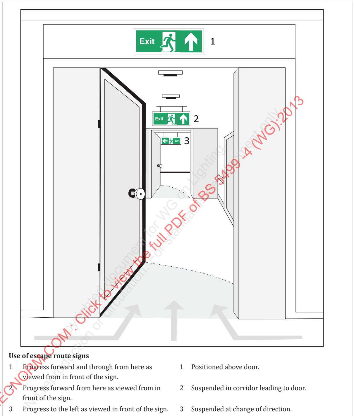
Figure A.12 — Typical connecting corridor with left turn juncture showing the correct use of escape route sign(s) and supplementary text
