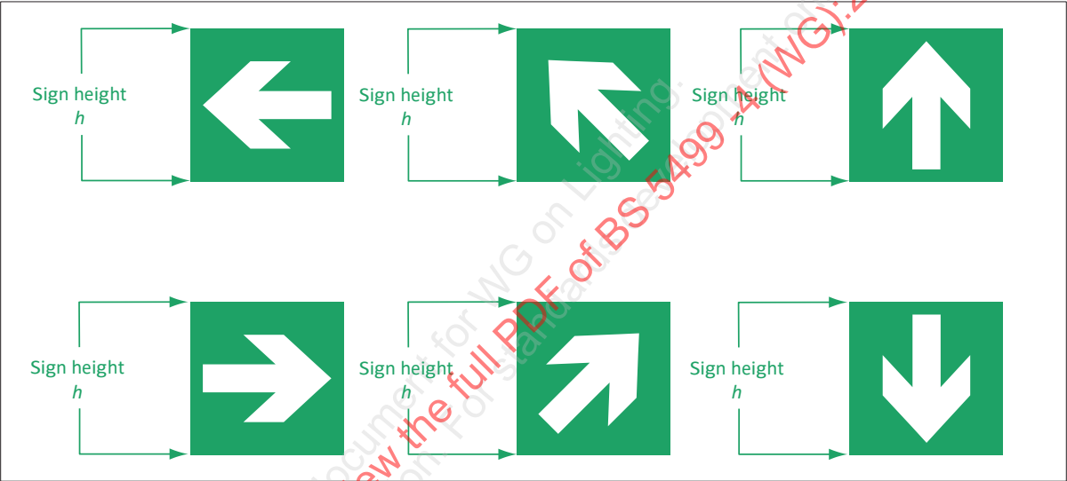
Figure 6 — Supplementary direction arrows
