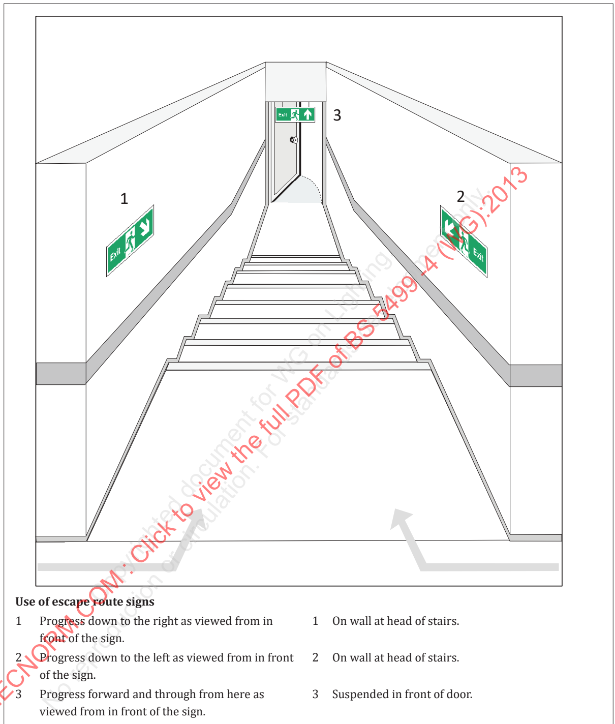
Figure A.4 — Typical single flight descent stairway showing the correct use of escape route sign(s) with supplementary text
