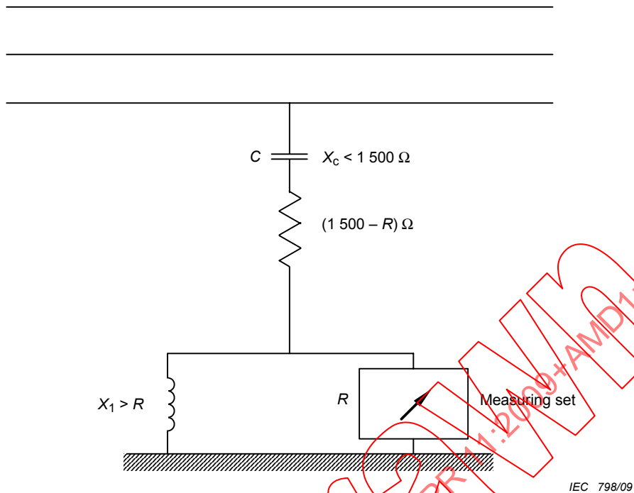
Figure 4 – Circuit for disturbance voltage measurements on mains supply (see 7.3.3)
