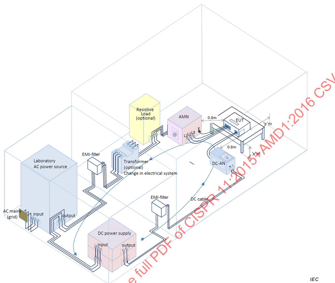
Figure J.2 – Setup of the test site (Case 1) – 3D diagram
