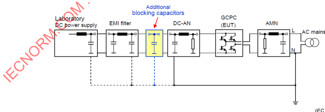
Figure K.3 – Blocking of flow of common mode RF current by employment of additional CM decoupling capacitors
