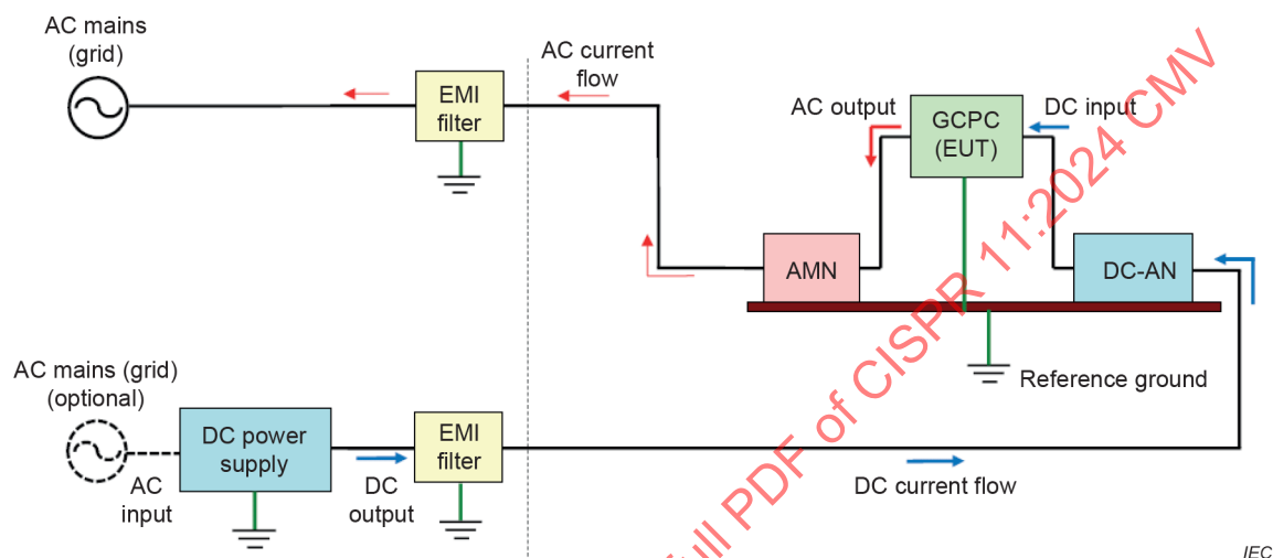
Figure D.5 – Setup of the test site (Case 3) – 2D diagram Test setup for Case 3 (schematic)
