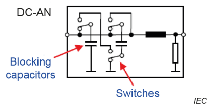
Figure E.7 – DC-AN circuit example where capacitance of blocking capacitors of the LC decoupling circuit can be increased or decreased
