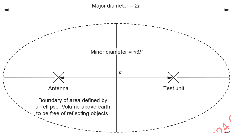
Figure 15 – Radiation test site
