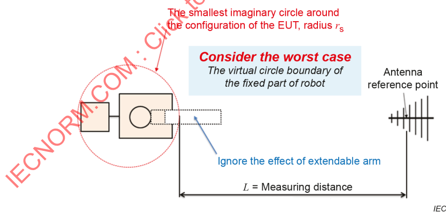
Figure 5 – EUT boundary determination for radiated disturbance measurements of robots with extendable/moving arm
