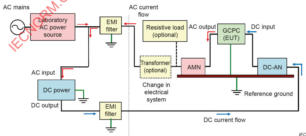
Figure D.1 – Setup of the test site (Case 1) – 2D diagram Test setup for Case 1 (schematic)
