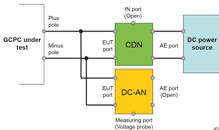
Figure 12 – Typical arrangement for measurement of conducted disturbances at LV DC power ports with the DC-AN used as termination and voltage probe
