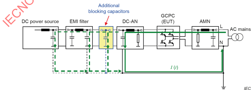
Figure E.5 – Prevention of saturation of mitigation filters by use of additional decoupling capacitors
