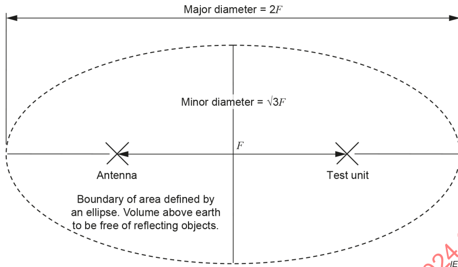
Figure 15 – Radiation test site
