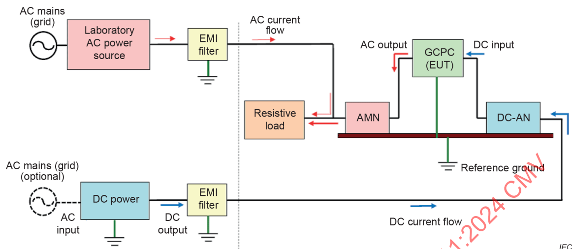
Figure D.3 – Setup of the test site (Case 2) – 2D diagram Test setup for Case 2 (schematic)
