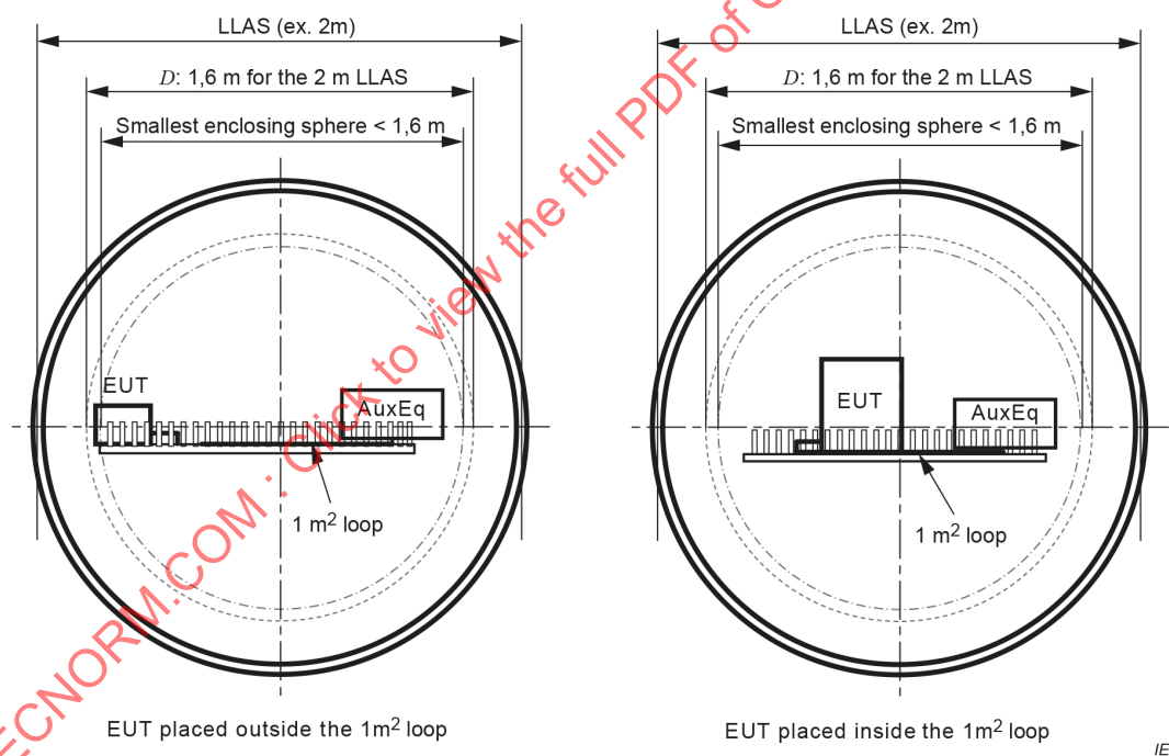
Figure C.6a – Top view
