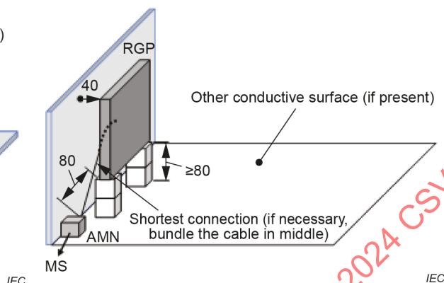
Figure B.4b – vertical RGP
