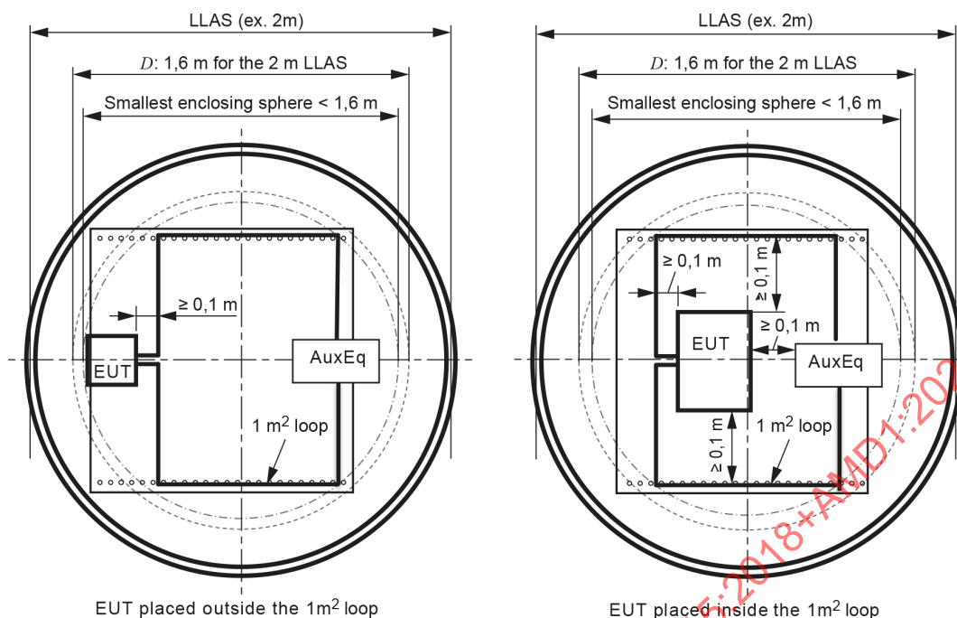
Figure C.6a – Top view
