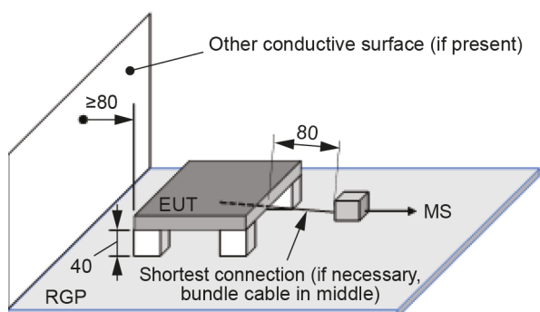
Figure B.4a – horizontal RGP
