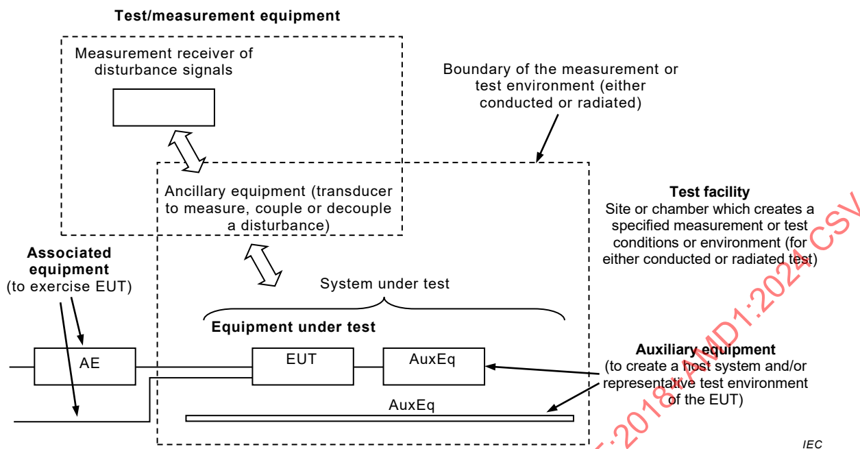
Figure 2 – Generic depiction of the definitions of test-, ancillary-, auxiliary- and associated equipment w.r.t. EUT and the test/measurement environment (definitions given in CISPR 16-2-3)
