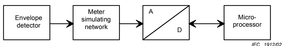
Figure 45 – Block diagram of an average detector.
