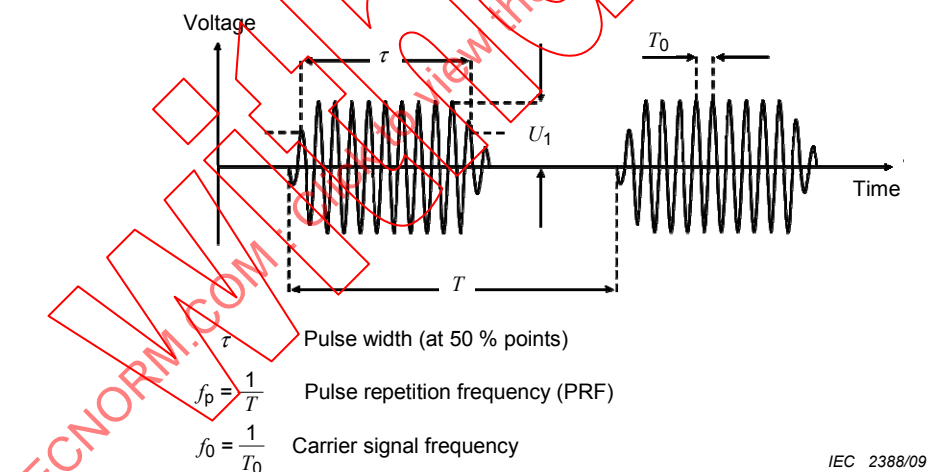
Figure E.4 – Pulse-modulated RF signal applied to a measuring receiver
