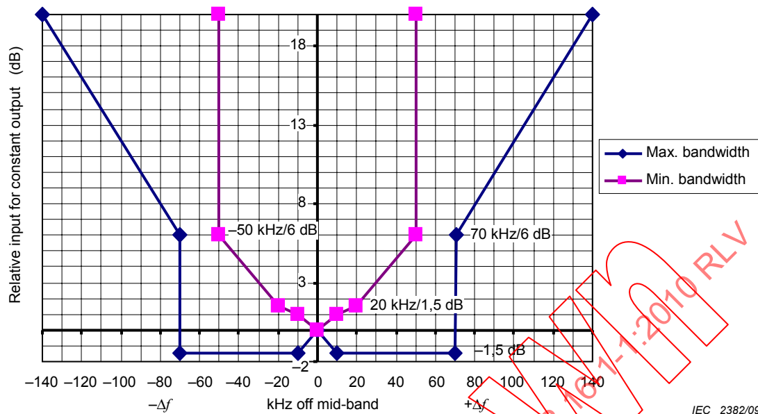
Figure 2c) – Limits of overall selectivity – Pass band (see 4.5.1, 5.55.6, 6.56.6, 7.57.6) (Bands C and D)
