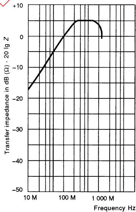
Figure B.3 – Transfer impedance of typical current probes (see clause B.4)
