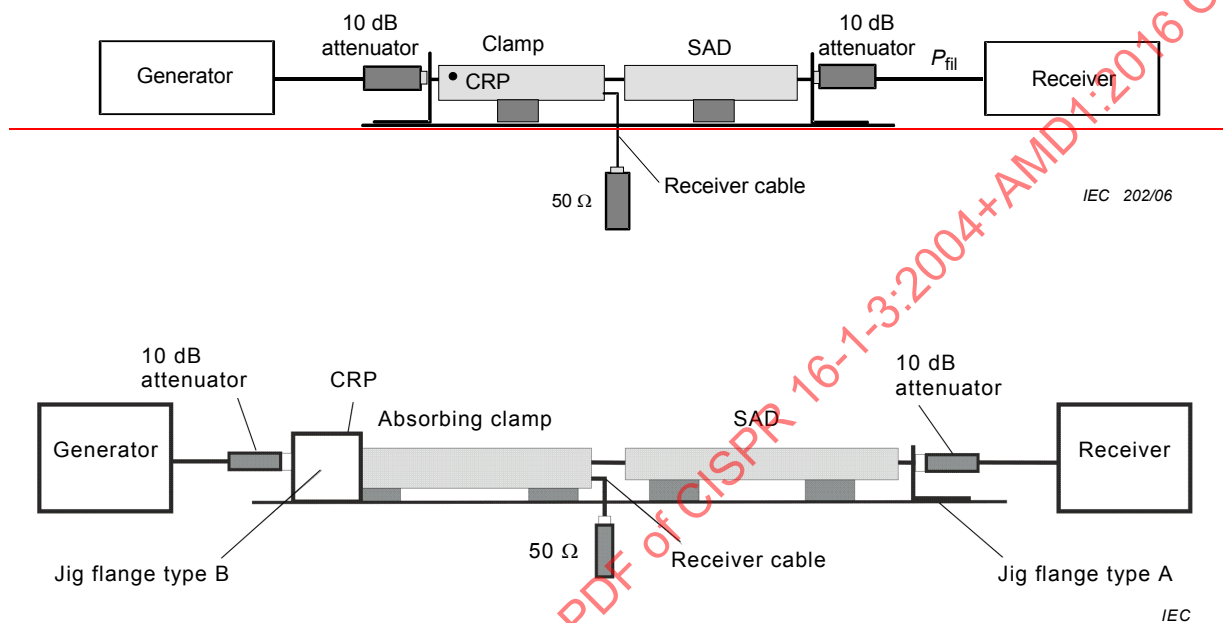
Figure B.8b – Measurement with the absorbing clamp and SAD placed in the jig
