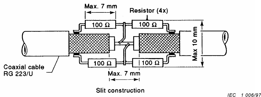
Figure C.3 – Construction of the antenna slit
