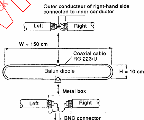
Figure C.9 – Construction of the balun-dipole
