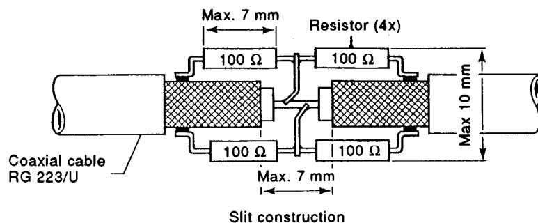
Figure C.3 – Construction of the antenna slit
