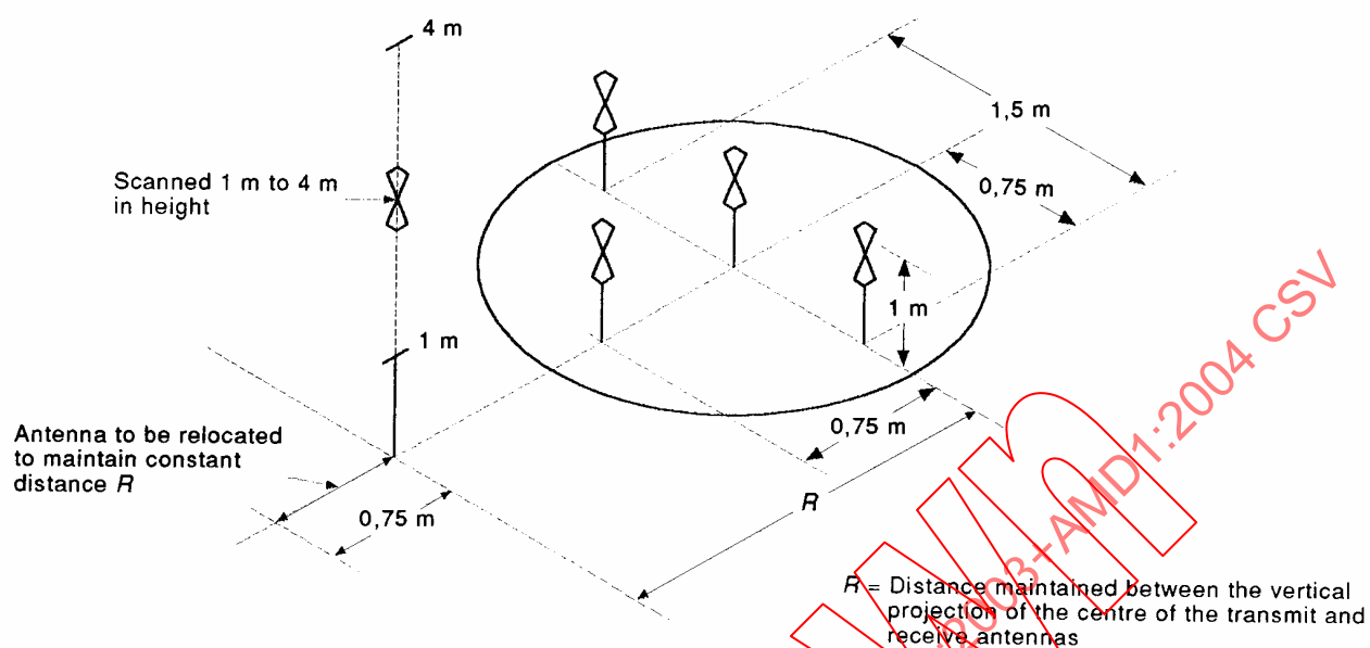
Figure 6c – Typical antenna positions for alternative test site – Vertical polarization NSA measurements for an EUT that does not exceed a volume of 1 m depth, 1,5 m width, 1,5 m height, with the periphery greater than 1 m from the closest material that may cause undesirable reflections
