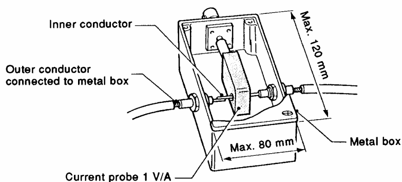
Figure C.5 – Construction for the metal box containing the current probe
