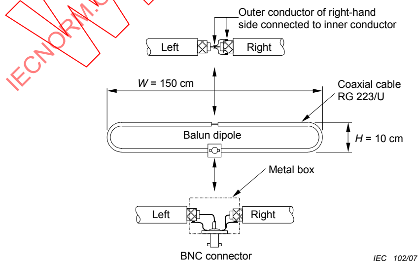
Figure C.9 – Construction of the balun-dipole
