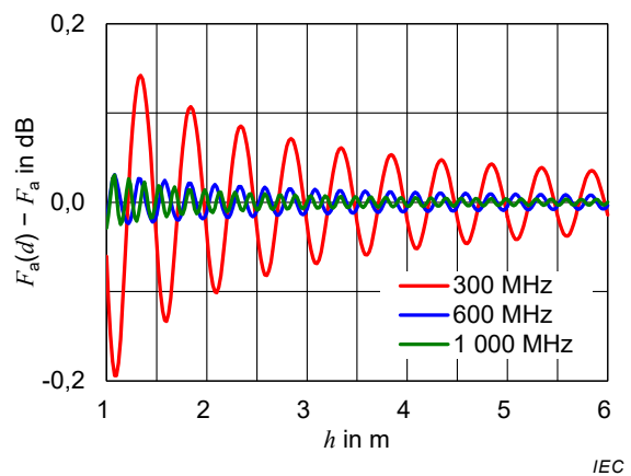
f) LPDA antenna ( Z'_0 = 50 \Omega ; horizontal polarization)
