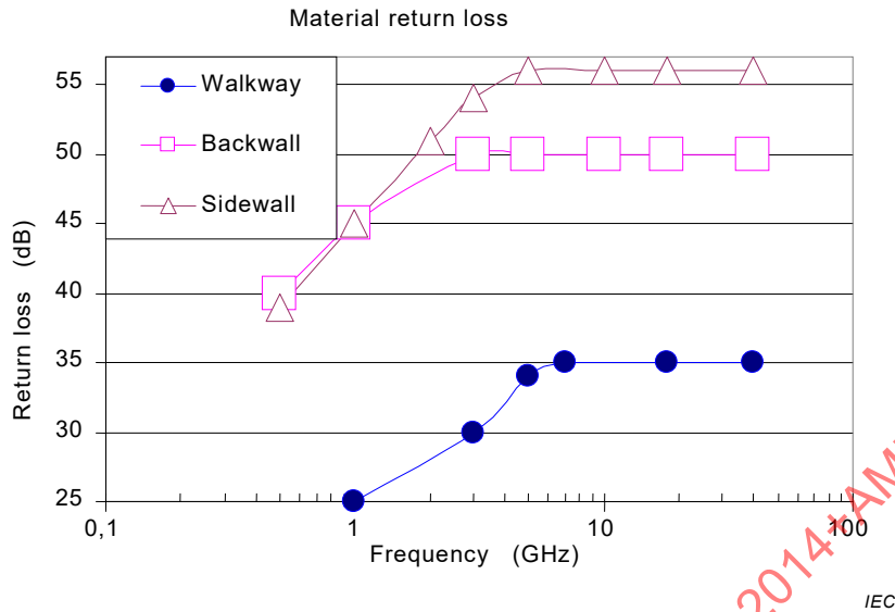
Figure E.3 – Reflectivity of chamber absorbing materials
