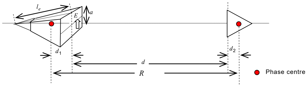
Figure 15 – Separation distance with respect to the phase centre of horn antennas (see [49] for details)
