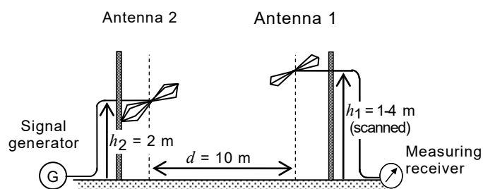
(a) Antenna pair (2,1)
