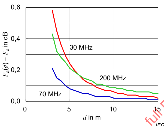
c) Biconical antenna ( Z'_0 = 200 \Omega )
