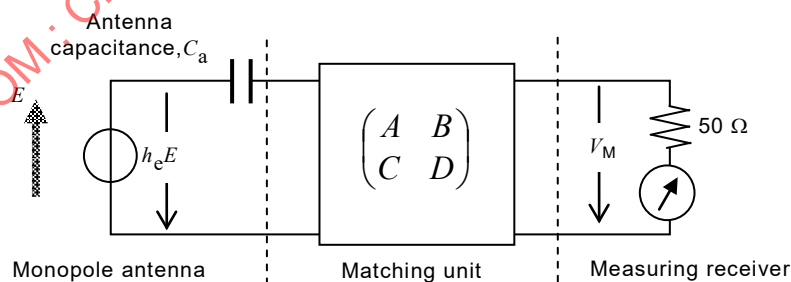
Figure G.6 – Equivalent circuit representation for a monopole antenna system
