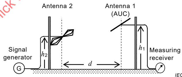
a) Antenna pair (2,1)
