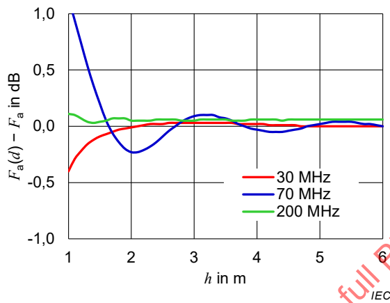
c) Biconical antenna ( Z'_0 = 50 \Omega ; vertical polarization)
