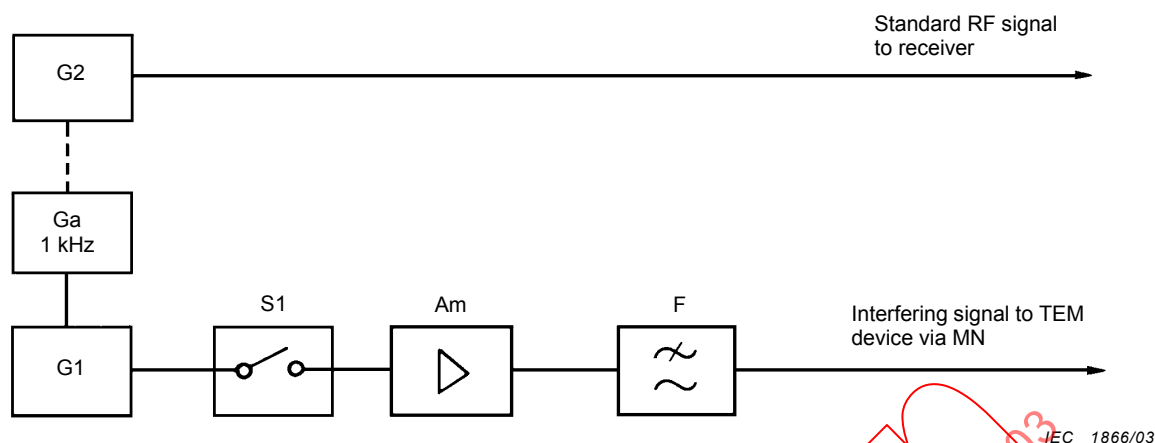
Figure 31 – Measuring circuit for the immunity of sound broadcast receivers to ambient fields (see 3.3.1.1.1)
