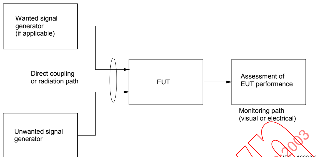
Figure 25 – Fundamental concept of immunity measurement (see 3.1.1)
