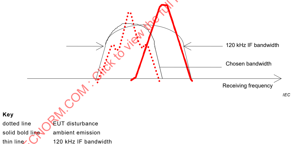
Figure A.4 – Disturbance by an amplitude-modulated signal (dotted line)
