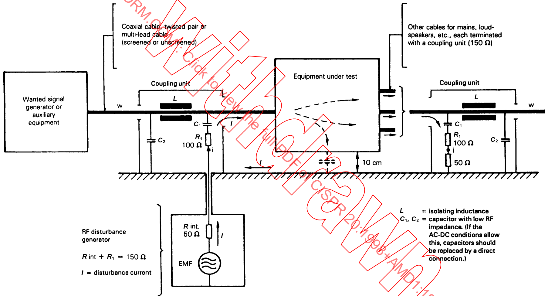
Figure 12 – General principle of the current-injection method (see 5.4.2)
