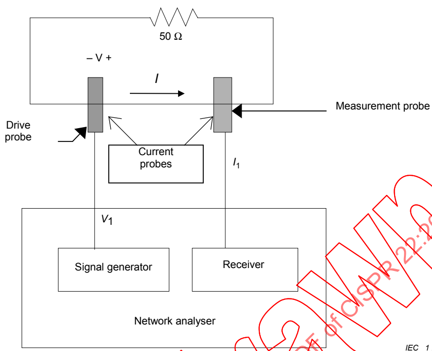
Figure C.5 – Calibration fixture
