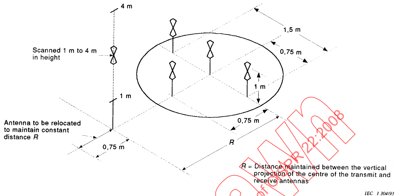
Figure A.2a – Typical antenna positions for alternate site NSA measurements in the vertical polarization for a volume not to exceed 1 m depth, 1,5 m width and 1,5 m height and rear boundary of the volume greater than 1 m from the closest material that may cause undesirable reflections
