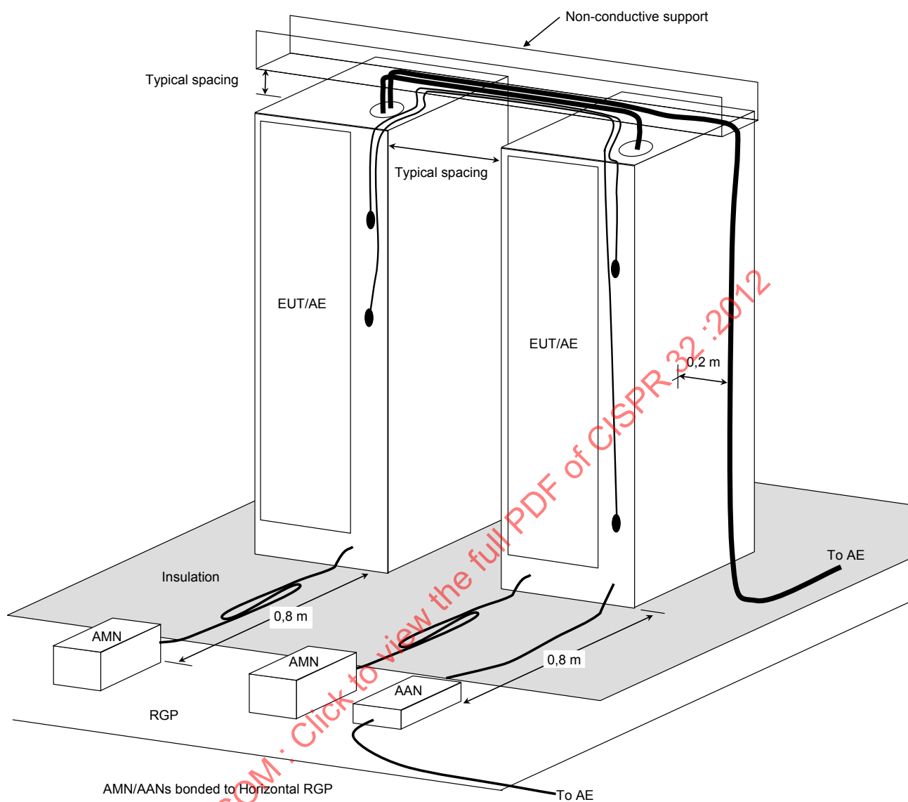
Figure D.6 – Example measurement arrangement for floor standing EUT (Conducted emission measurement)
