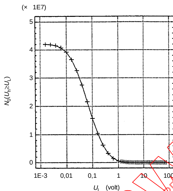
Figure 4.4.4-3 – Example of the number of outlets with an induced asymmetrical open-circuit voltage U_L \leq U_h \leq U_{\max} = 79 V, see table 4.4.4-1. Total number of outlets N_T = 42 \cdot 10^6
