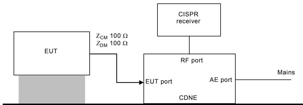
Figure 205 – Block diagram for CDNE-measurement method
