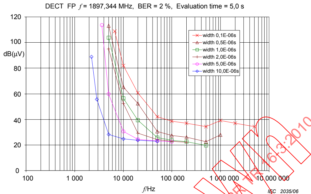
Figure 163 – Weighting characteristics for DECT (signal level –83 dBm)
