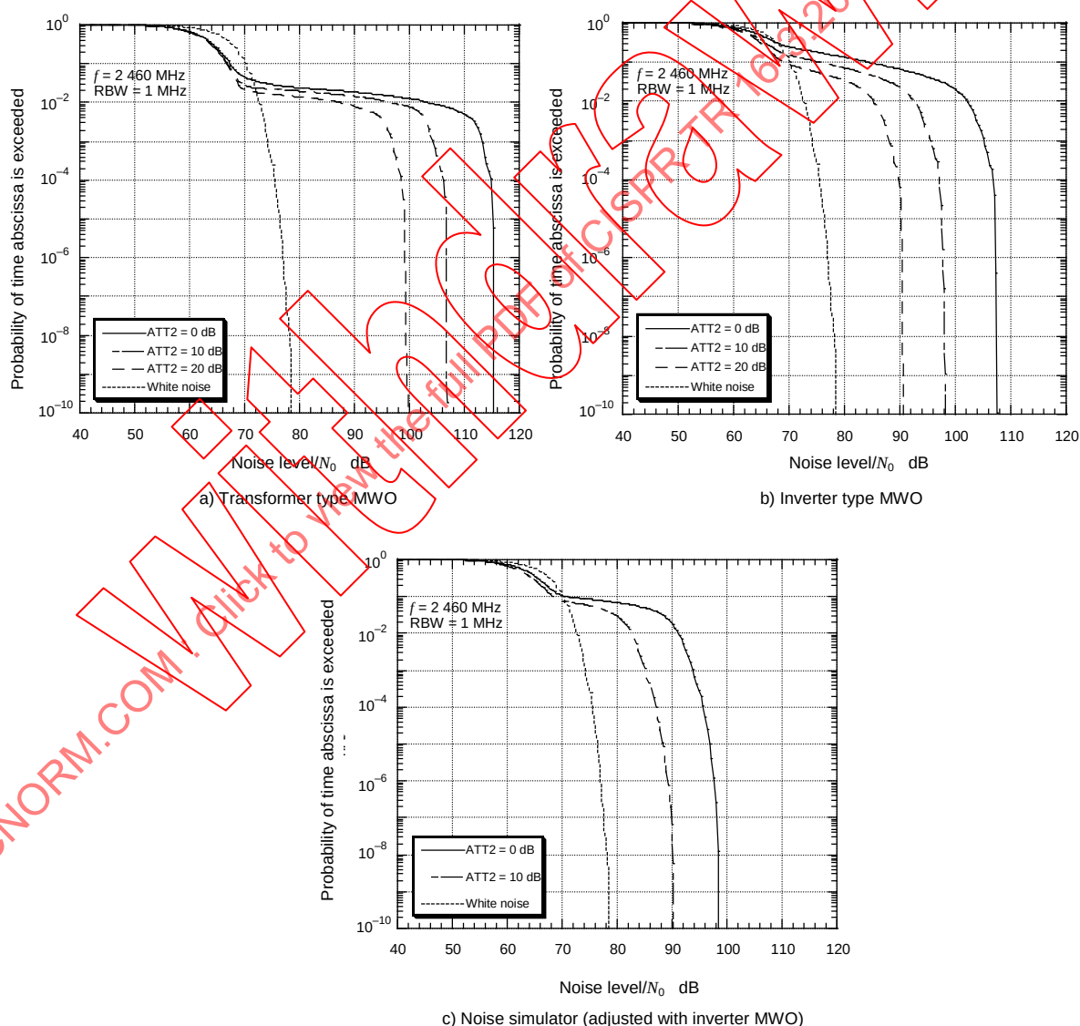
Figure 118 – APD characteristics of disturbance (2 460 MHz)
