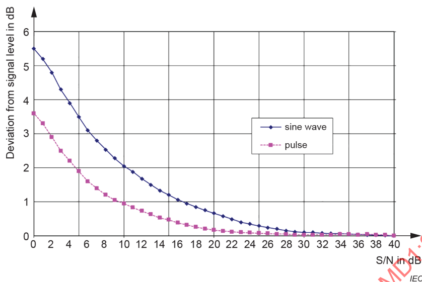
Figure D.7 – Deviation of the peak detector level indication from the signal level at receiver input for two cases: sine-wave signal, and impulsive signal (PRF 100 Hz)
