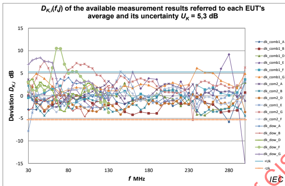
Figure C.8 – Deviation of the conversion factors from the average conversion factor of each EUT
