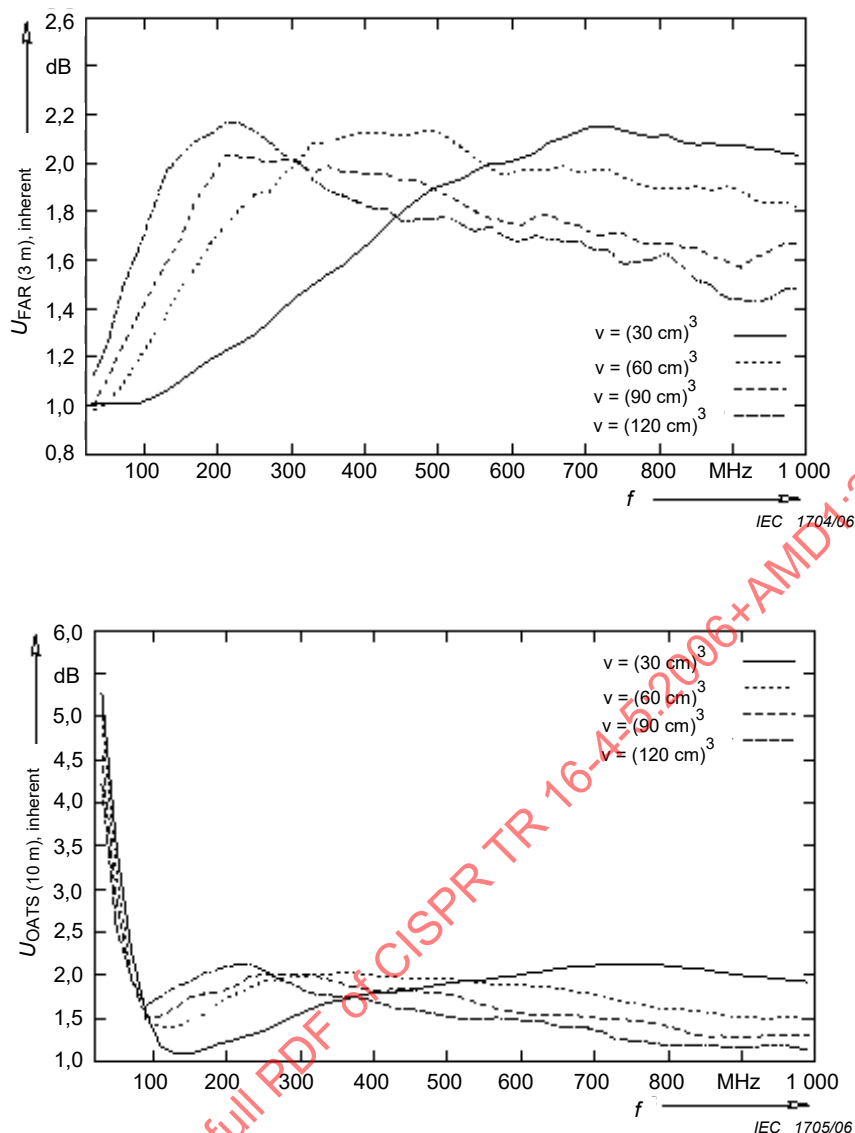
Figure B.7 – Uncertainties due to the unknown EUT characteristic for 3 m FAR (top) and 10 m OATS (bottom)
