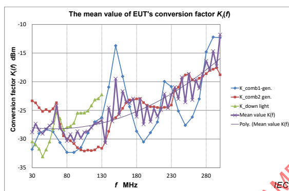
Figure C.5 – Mean conversion factors for each EUT
