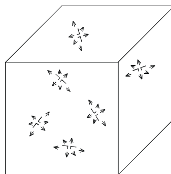
Figure B.4 – Radiation characteristics of elementary radiator (left), and scheme of EUT-model (right)
