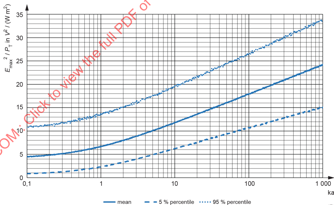
Figure D.5 – Conversion factor (mean and quantile values) from FSOATS/FAR results to RC results for d = 3 m measurement distance as a function of electrical EUT size ka
