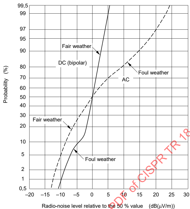
Figure 12 – Example of typical statistical yearly "all-weather" distributions of the radio-noise levels of a bipolar direct current line (—) and for an alternating current line in a moderate climate (- - -)
