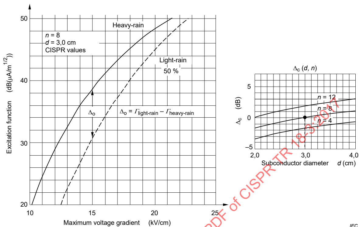
Figure 1 – Bundle conductors
