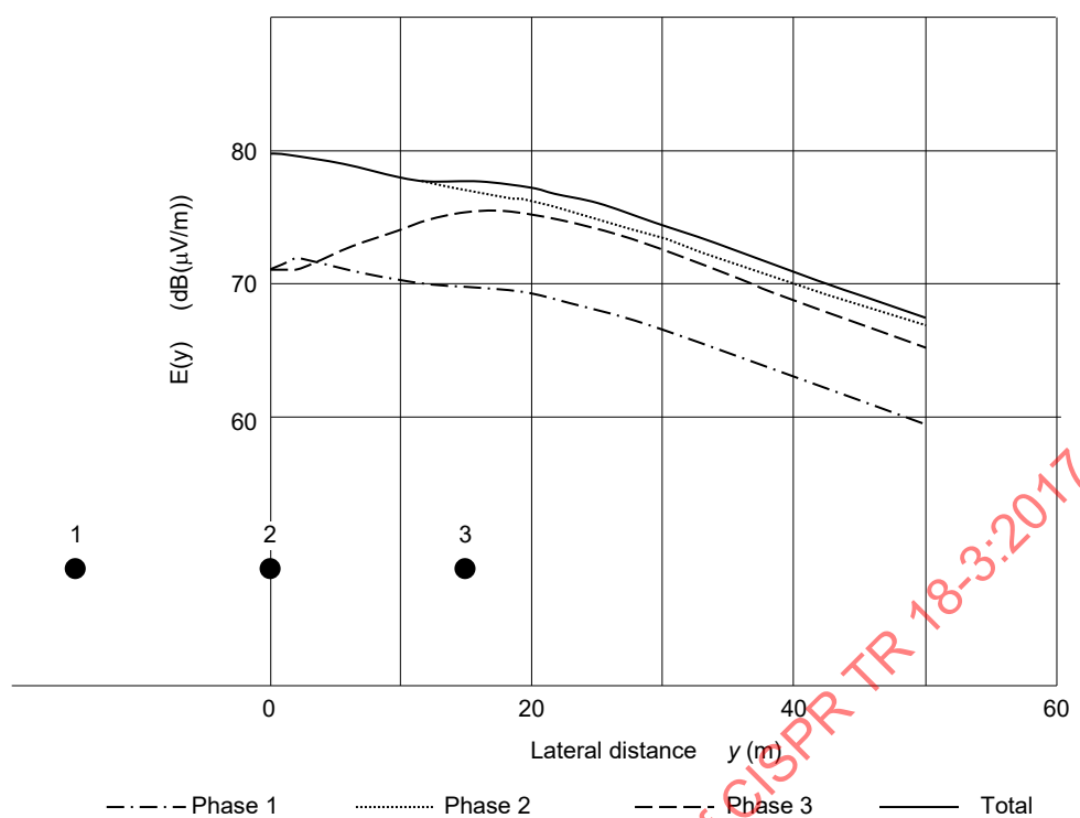
Figure C.2 – Lateral profiles of the radio noise field strengths produced by the individual phases and of the total field, as calculated in the given example
