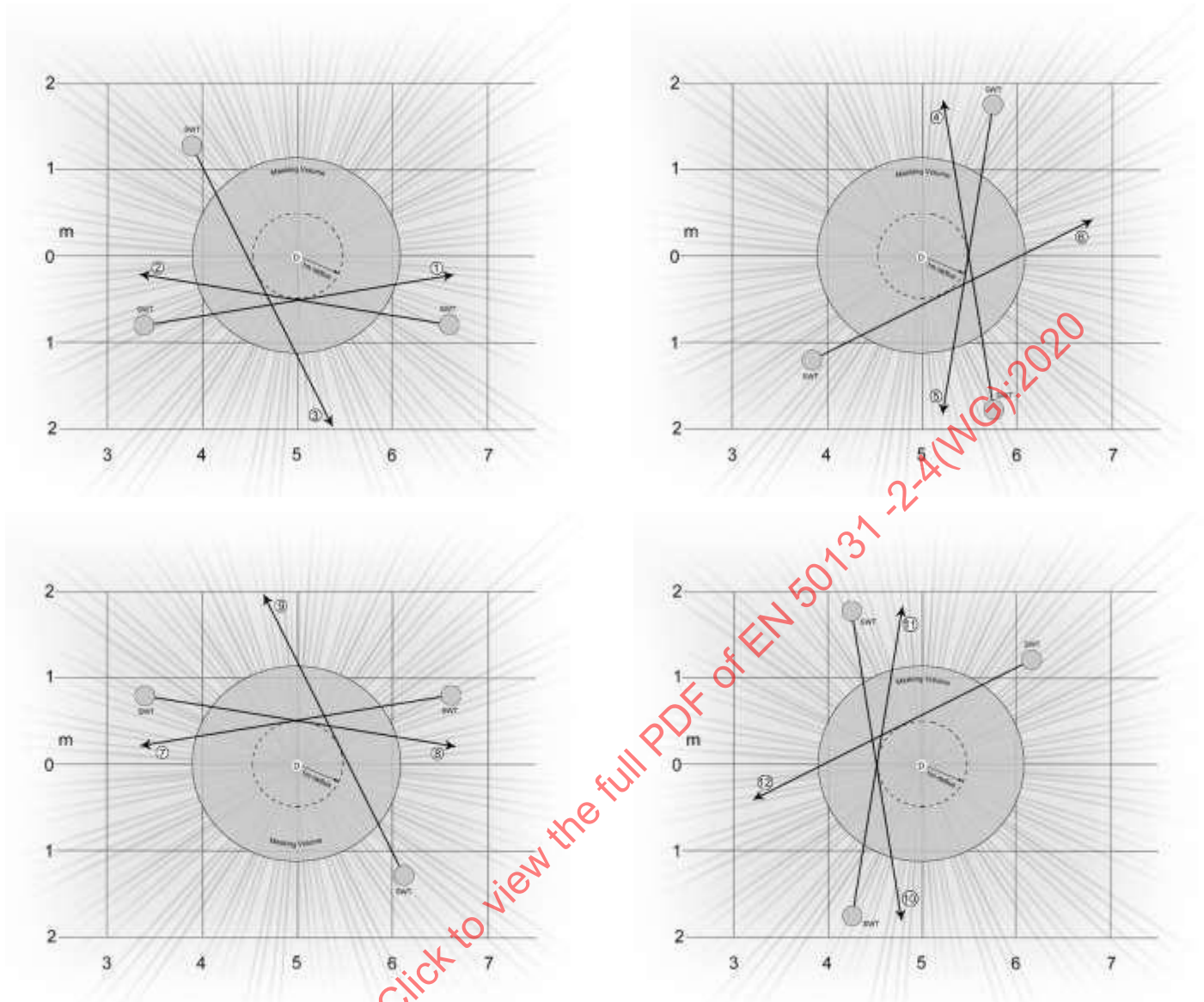
b) Immunity to False Masking signals for detectors with a 360° coverage angle (6.8.6)
