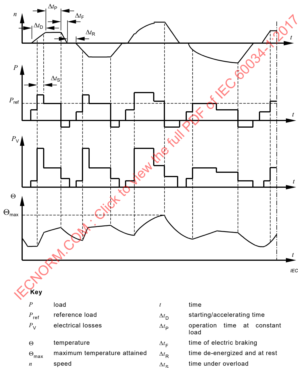
Figure 9 – Duty with non-periodic load and speed variations – Duty type S9
