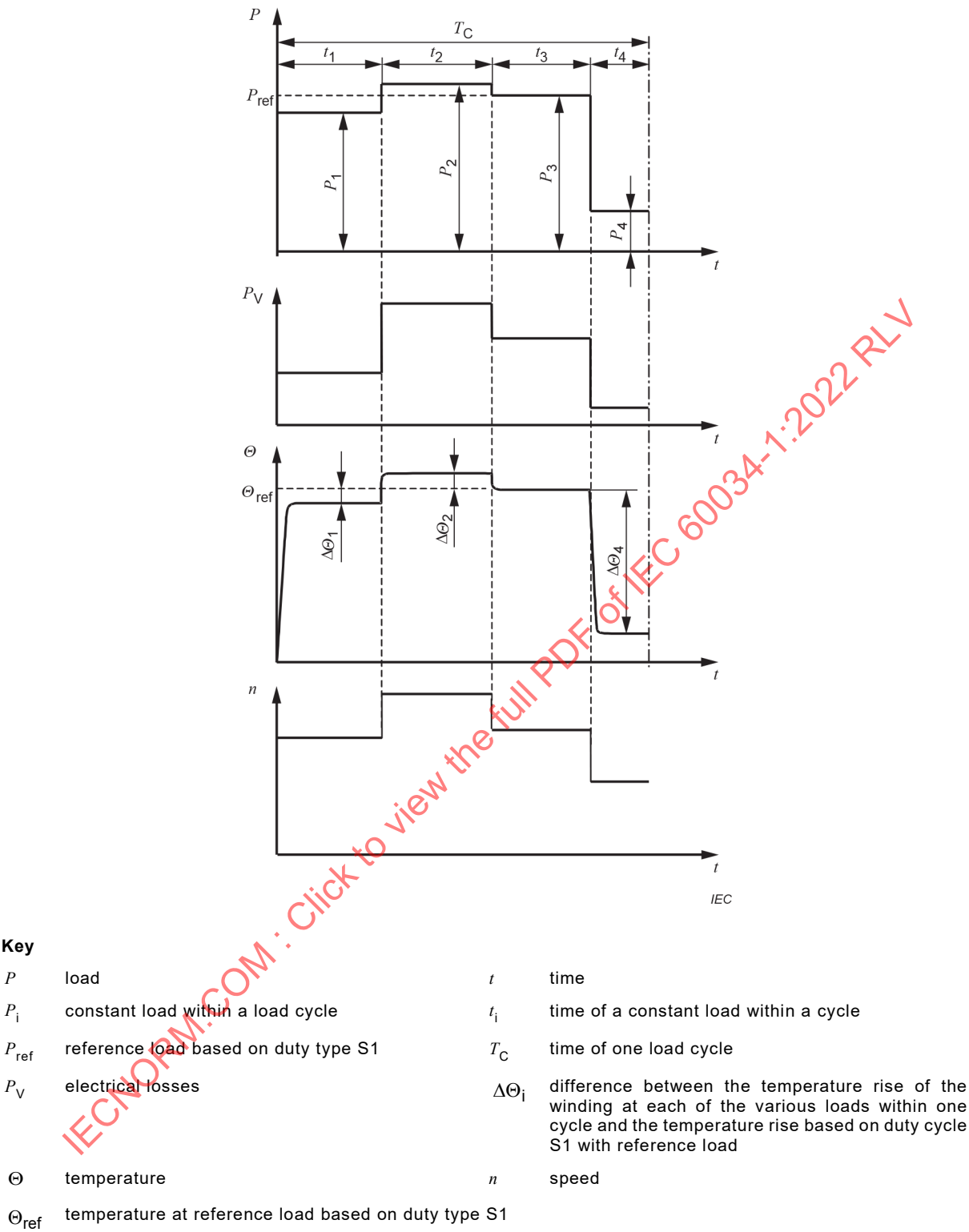
Figure 10 – Duty with discrete constant loads – Duty type S10
