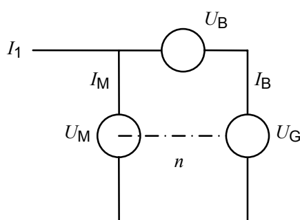
Figure 3 – Sketch for single supply back-to-back test, d.c. machines
