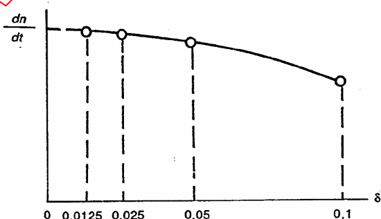
Figure D.2 – Method of the limiting secant
