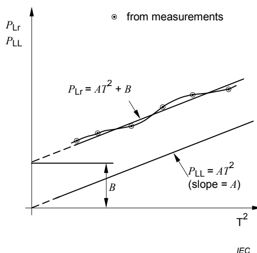
Figure 10 – Smoothing of the residual loss data
