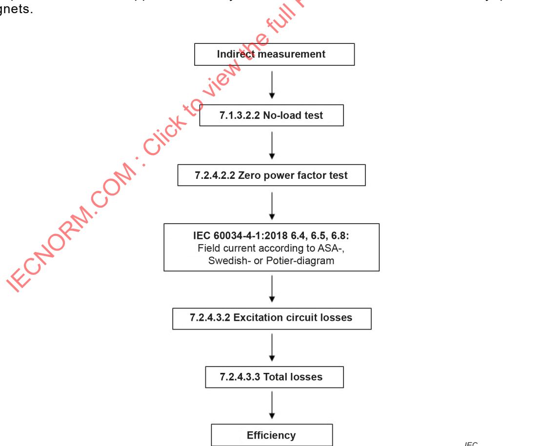
Figure 26 – Efficiency determination according to method 2-1-2F
