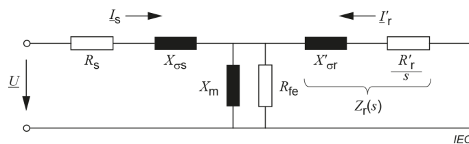
Figure 15 – Induction machine, T-model with equivalent iron loss resistor
