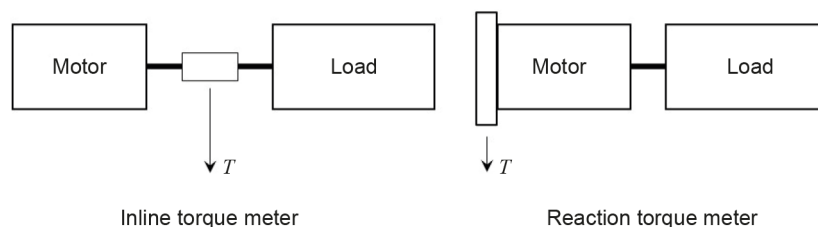
Figure 1 – Torque measuring devices
