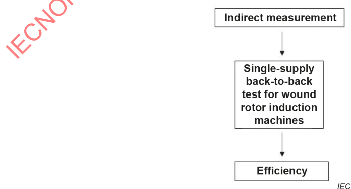
Figure 11 – Efficiency determination according to method 2-1-1E
