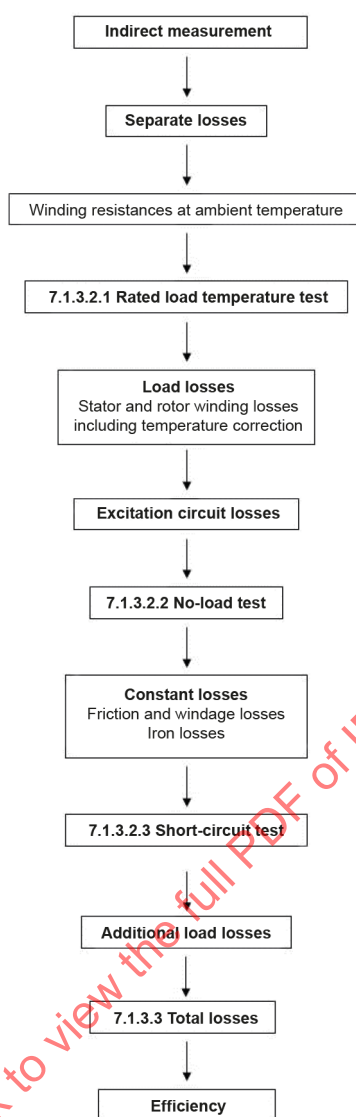
Figure 20 – Efficiency determination according to method 2-1-2B
