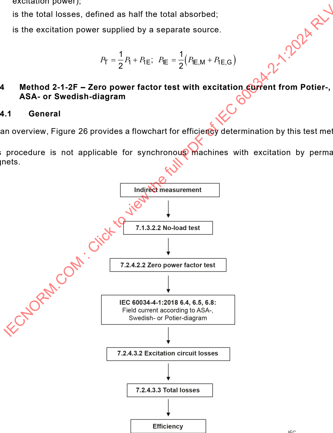
Figure 26 – Efficiency determination according to method 2-1-2F
