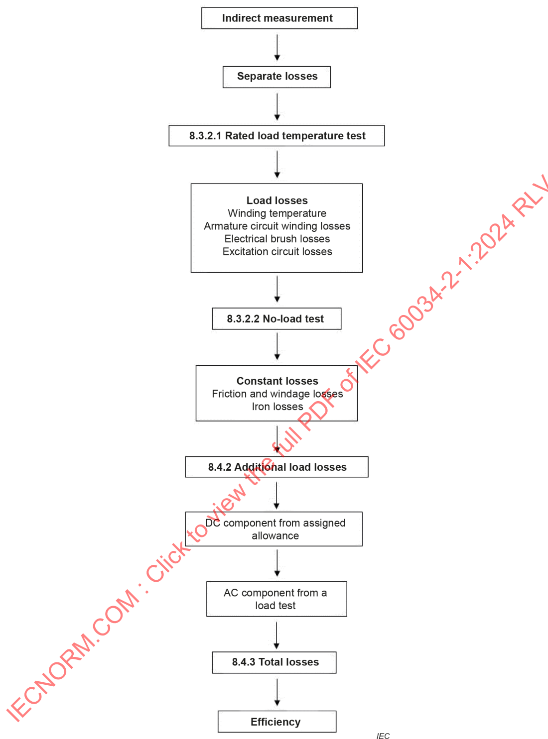
Figure 32 – Efficiency determination according to method 2-1-3C
