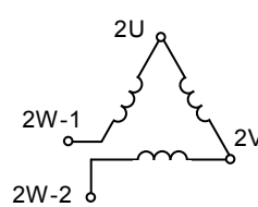
Figure A.15 – Constant-torque, seven terminals
