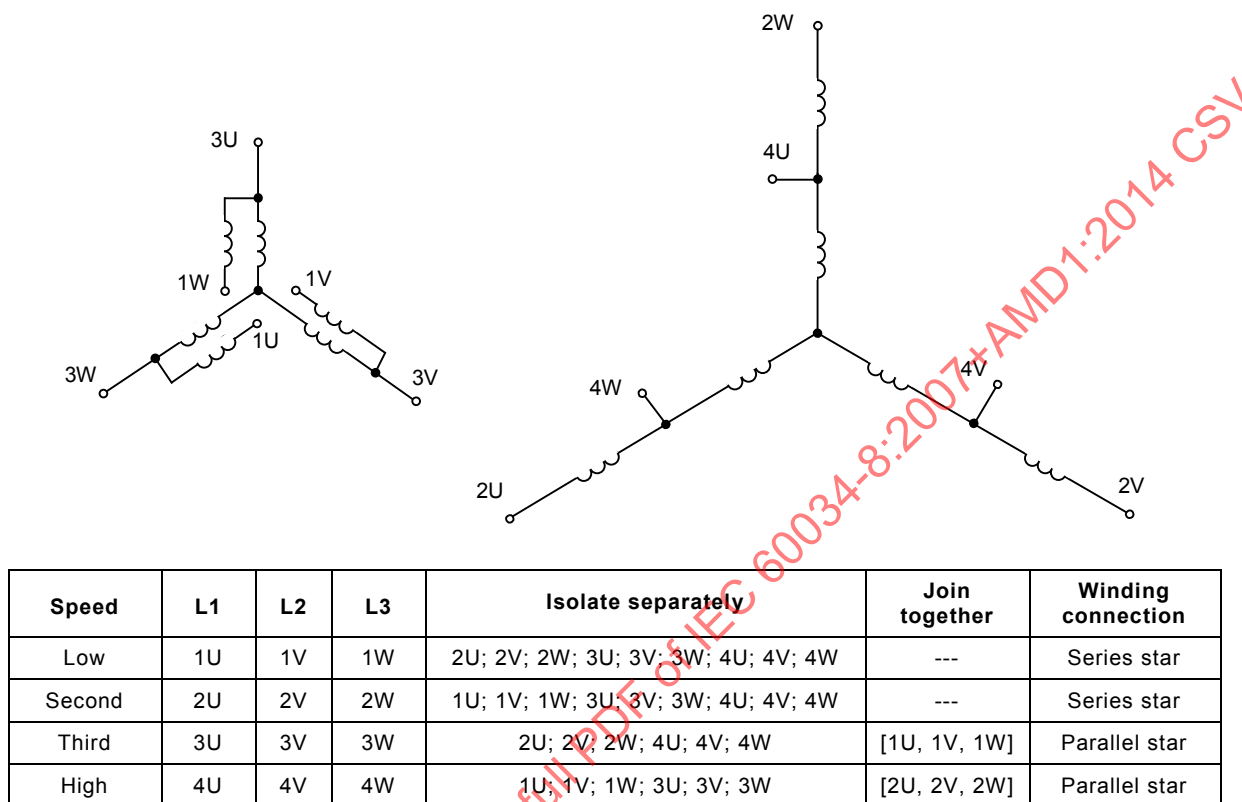
Figure A.19 – Example of four-speed, variable-torque motor using two separate windings, twelve terminals
