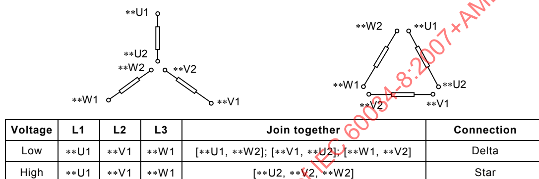
Figure 28 – Three-phase dual voltage
