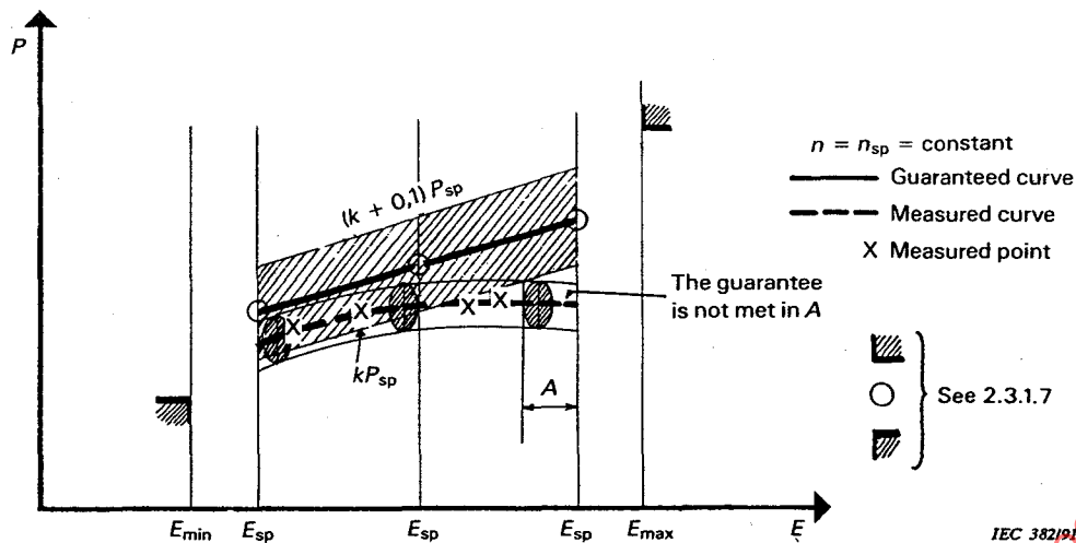
Figure 16 – Non-regulated turbine
