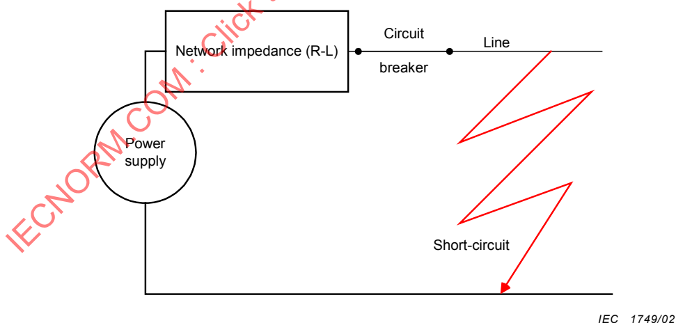
Figure A.1 – Equivalent electrical circuit of the network
