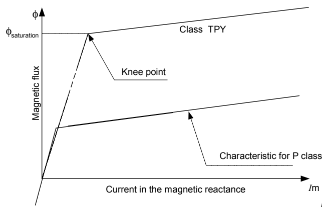
Figure A.7 – Example of the magnetic reactance of a CT for a TPY class
