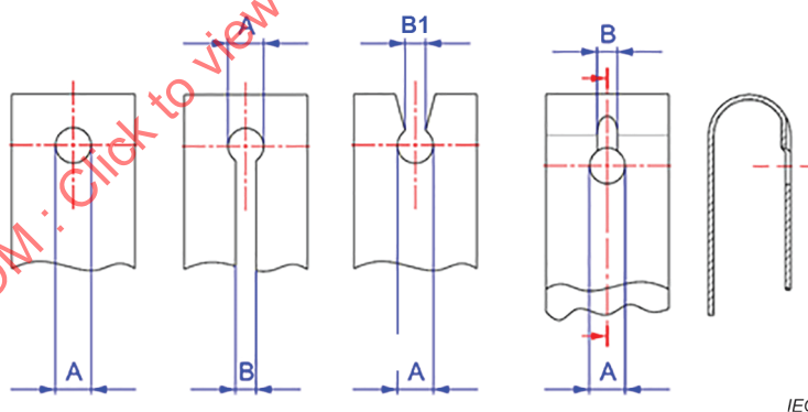
Figure 3 – Design examples (6) for SV7 and SV8.5 lampholder-contacts / Exemples de conception (6) de contacts des douilles SV7 et SV8.5
