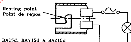
BA15d, BAY15d &amp; BAZ15d
