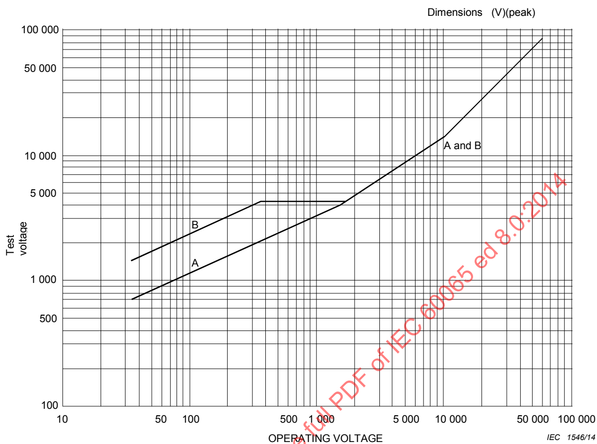
Figure 7 – Test voltages
