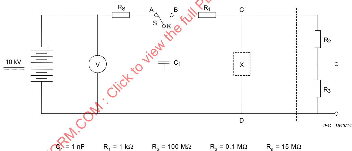
Figure 4 – Test hook
