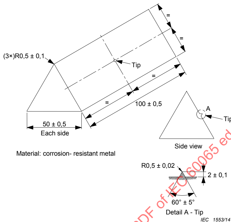
Figure 14 – Mandrel
