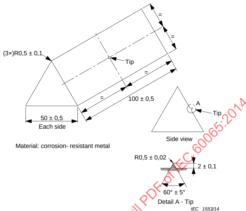
Figure 14 – Mandrel
