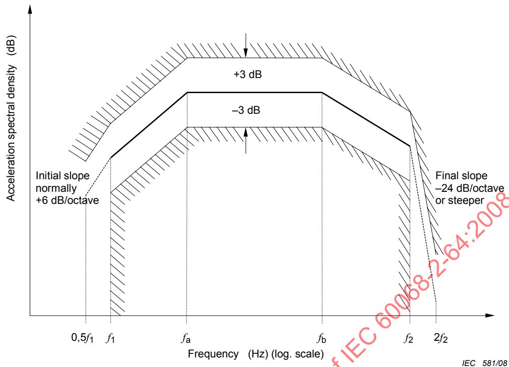
Figure 1 – Tolerance bands for acceleration spectral density; initial and final slope (see B.2.3)
