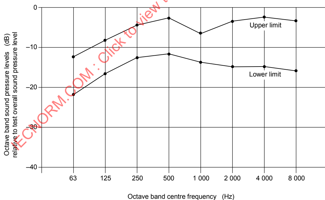
Figure 2 – Octave band spectra for fans derived from [4]
