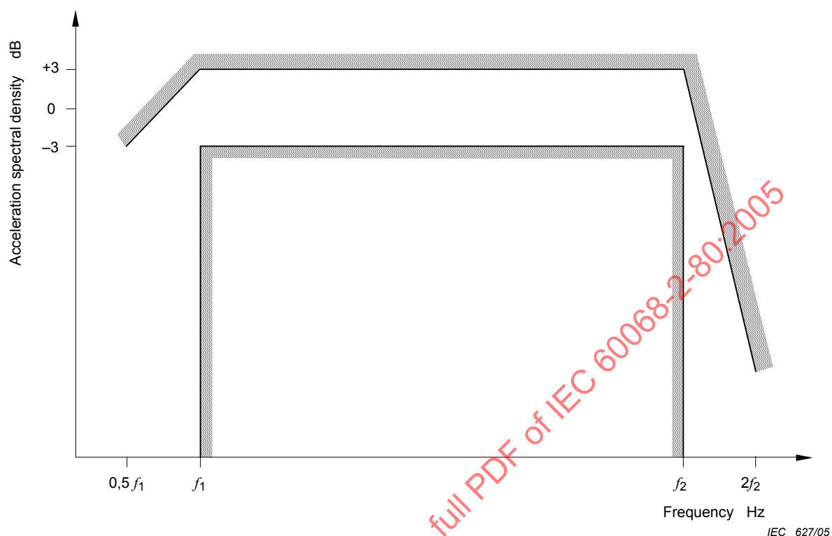
Figure 1 – Boundaries for acceleration spectral density (see also 5.1.1)
