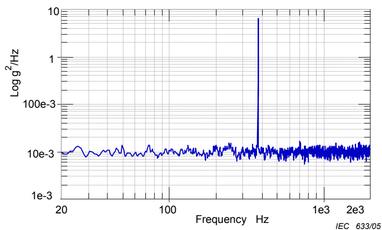
Figure A.2 – Sine at 380 Hz
