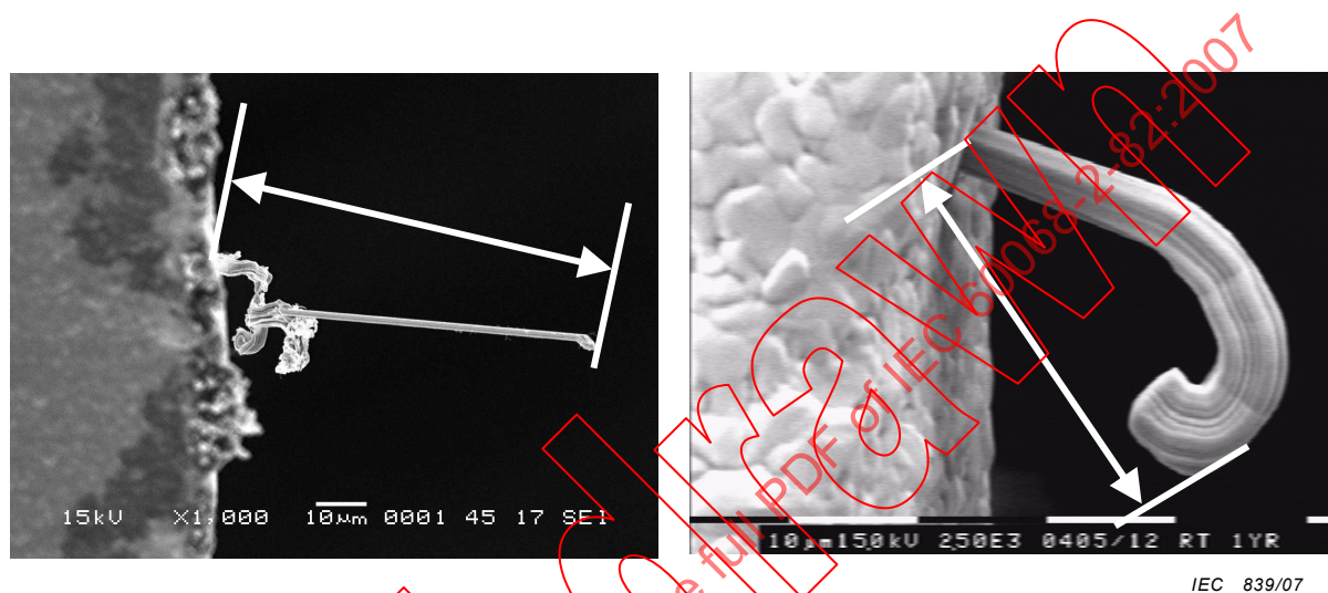
Figure A.1 – Definition of the whisker length
