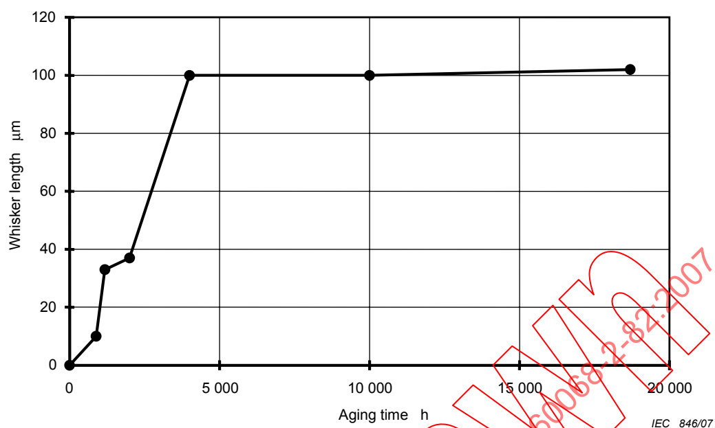
Figure F.1 – Whisker growth of tin plating in ambient test condition
