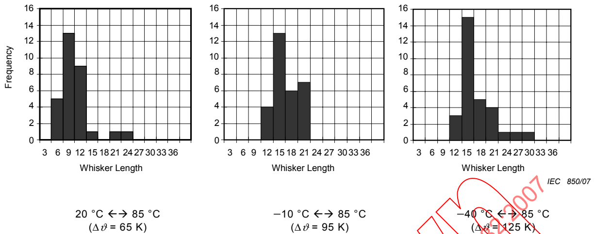
Figure H.1 – Distribution of whisker length grown on FeNi (Alloy42) base material
