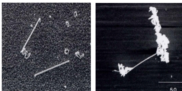
Figure B.3 – Filament whisker
