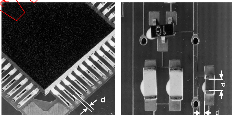
Figure D.1 – Smallest distance of components and circuit boards
