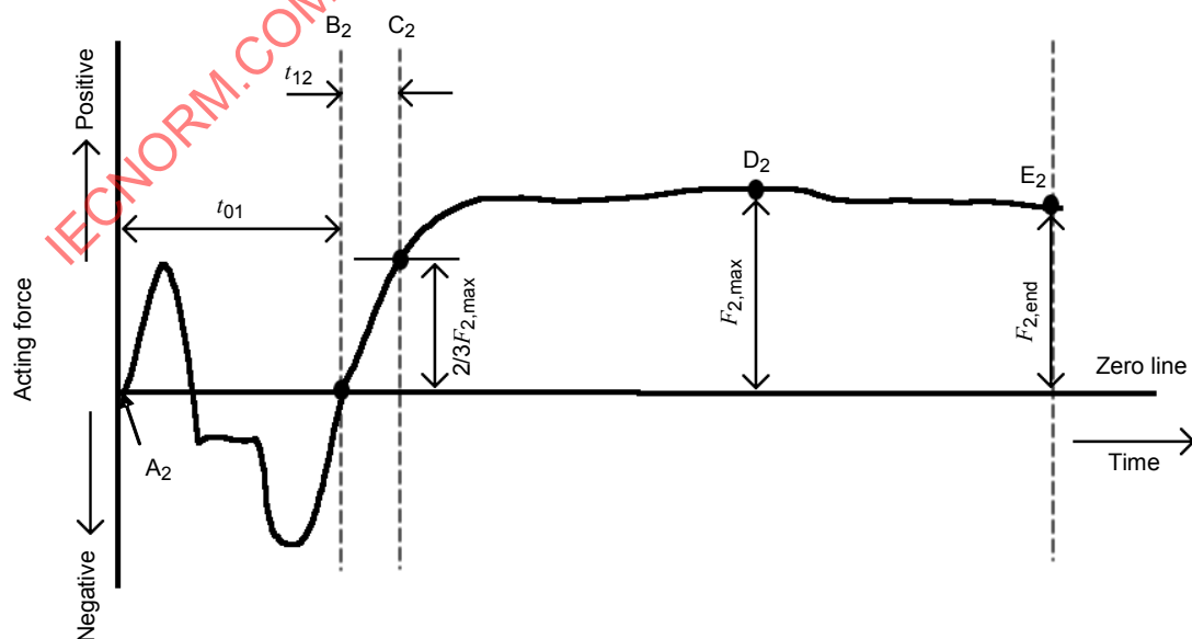
Figure E.3 – Showing the wetting force (pull) of some solder pastes
