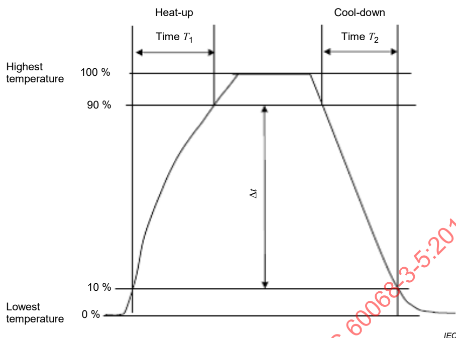
Figure 10 – Example of temperature rate of change for heating and cooling of a test chamber
