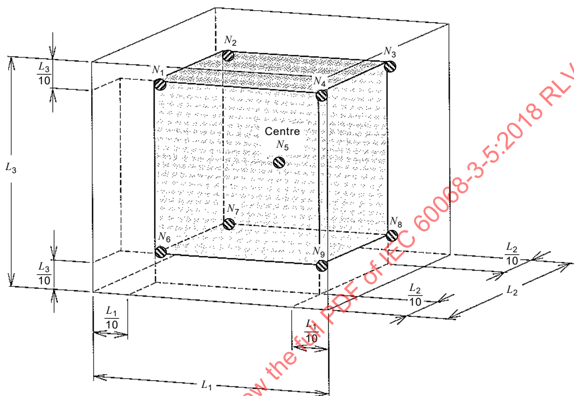
Figure 3 – Location of air temperature sensors for temperature chambers up to 2 000 l
