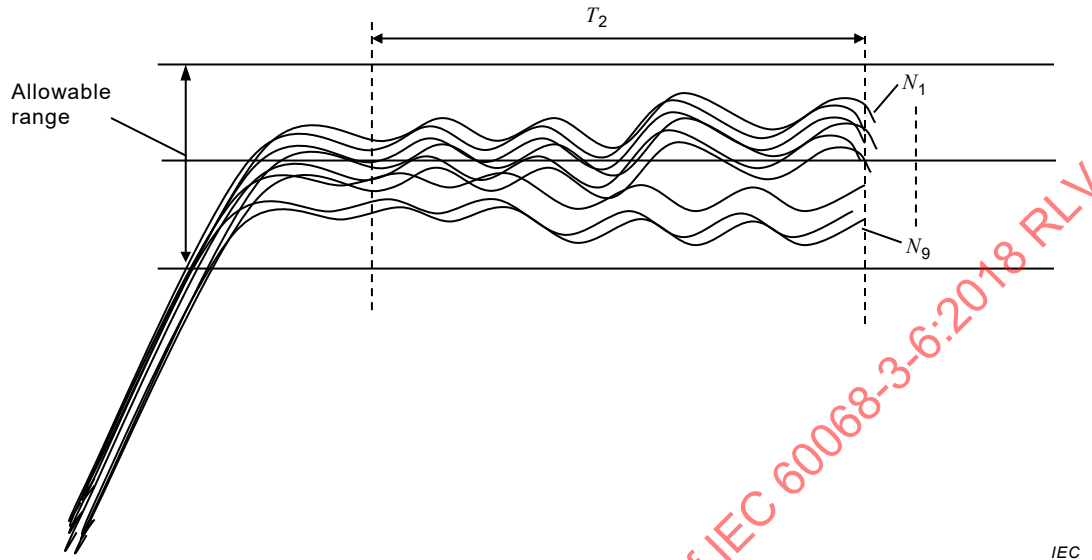
Figure 6 – Example of temperature/humidity stabilization
