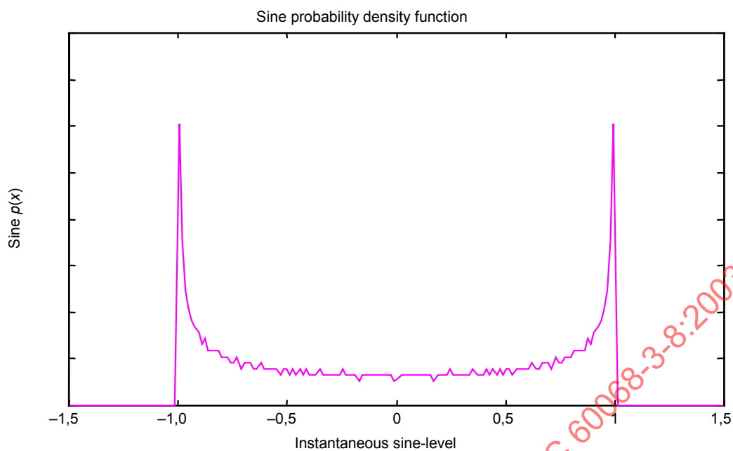
Figure 1 – Probability density of a single frequency sinusoidal signal
