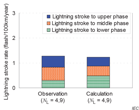
(b) 500-kV transmission lines
